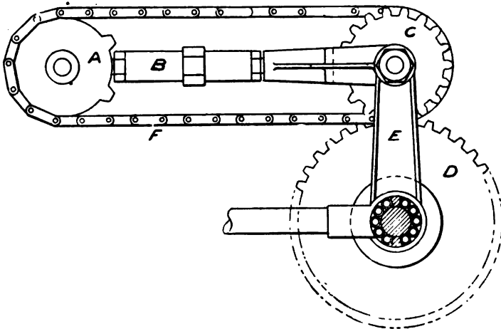
FIG. 335.—The Haynes-Apperson Transmission. A is the sprocket fixed at one end of the counter shaft; B, a turnbuckle on the adjustable distance rod between the first counter shaft and the second counter shaft carrying the pinion, C; C, a spur pinion keyed to the second counter shaft, carrying a sprocket driven by a chain from A; D, a spur gear on the rear axle meshing with spur pinion, C, on the second countershaft; E, a rigid distance rod for maintaining fixed relations between the spurs, C and D. The advantages of this system are the maintaining of a steady drive without the usual wear and tear on the moving parts, consequent on sprocket connections direct from the first countershaft, or from the main shaft of the motor.
